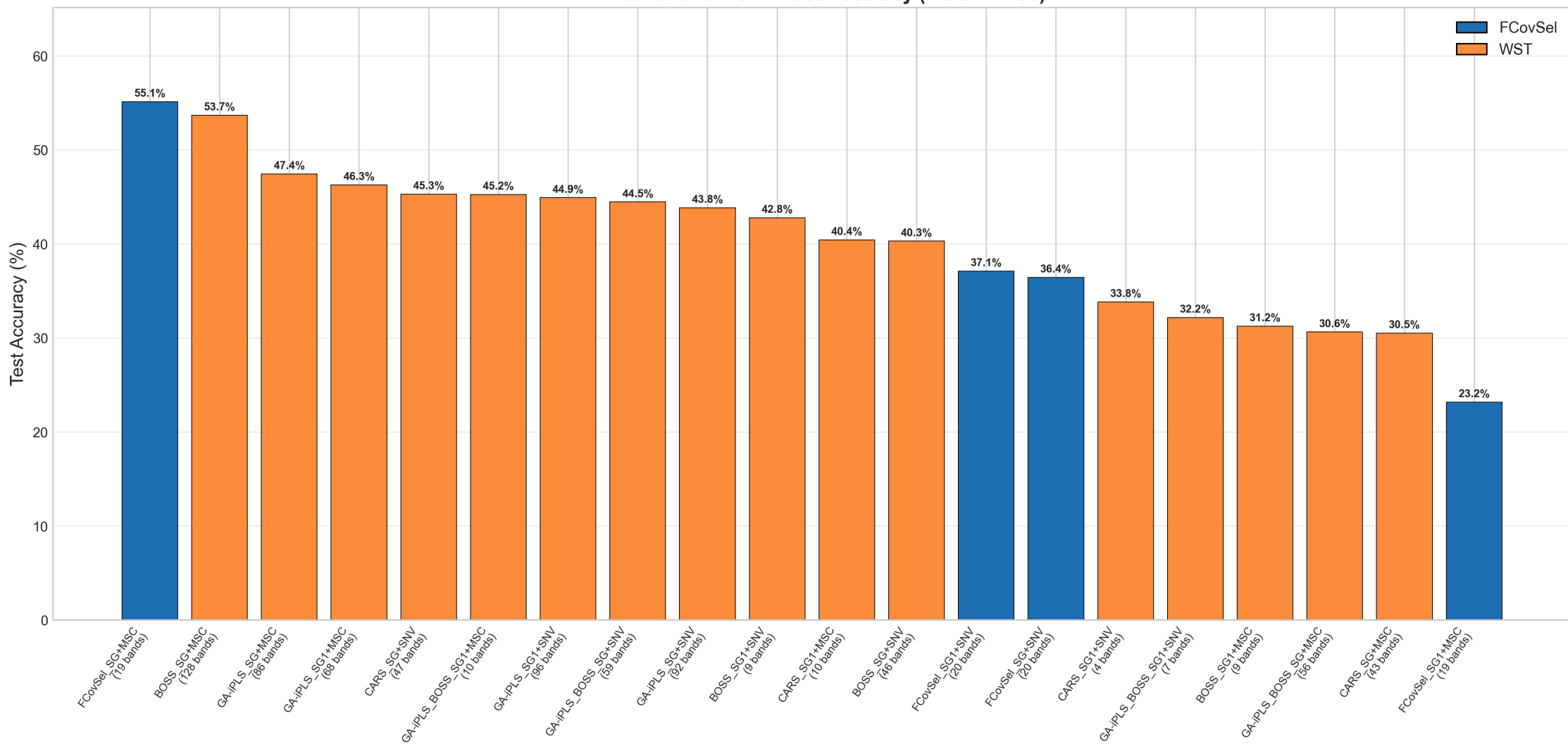
All Methods - 3D-CNN Test Accuracy (Indian Pines)
